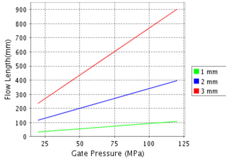
CALCULATED FLOW LENGTH INDICATION Moldflow® Radial Flow Analysis Valox® V3001MC Melt Temperature : 260°C Mold Temperature : 70°C
